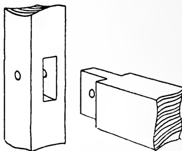
PINNED MORTISE &amp; TENON
